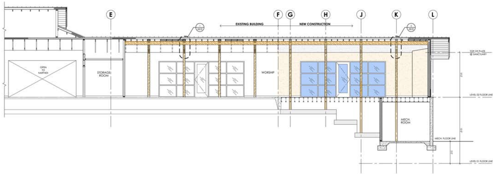
1 BUILDING SECTION A3/02 1/4" = 1'-0"
